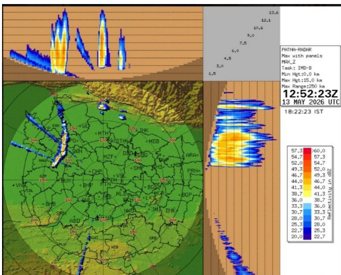
Fig-4(a-h): RADAR Images of Thunderstorm Event
