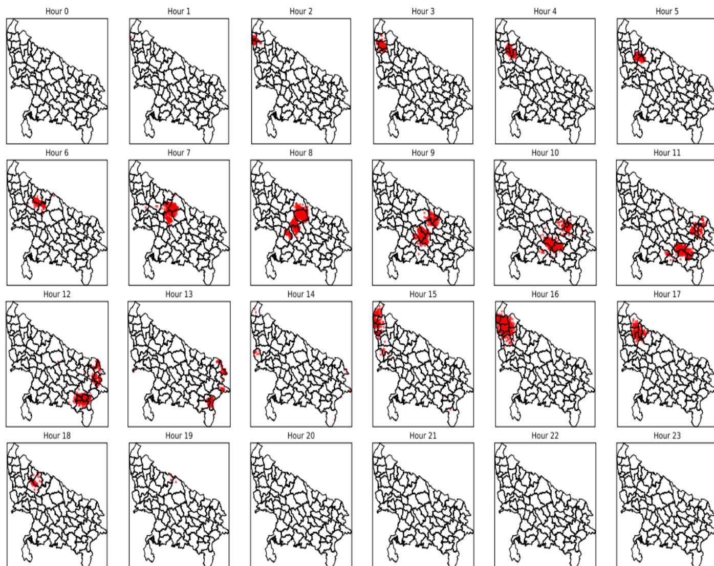
Fig-3 (b): District wise Hourly Total Lightning Strike count over UP
