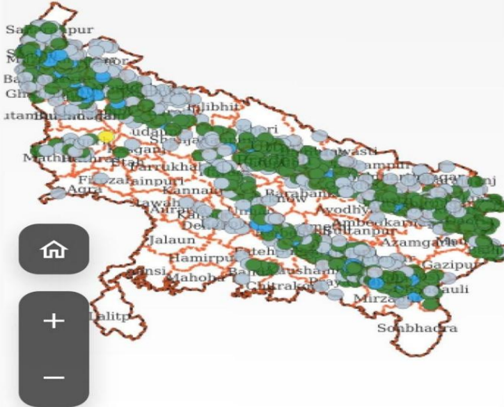
Fig-1 (a) Realized Station Rainfall over UP
