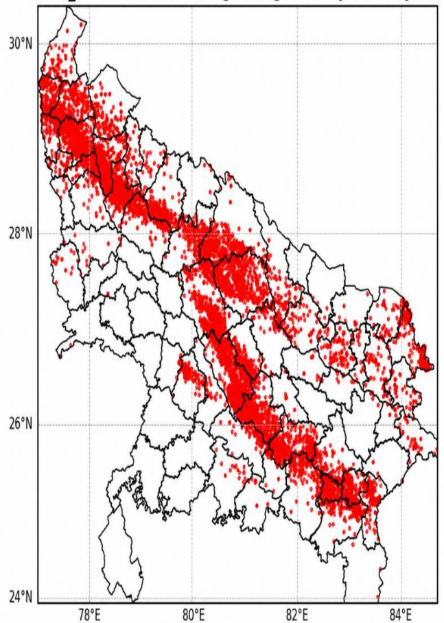
Fig-3(a) Total Realized Lightning strike count over UP
