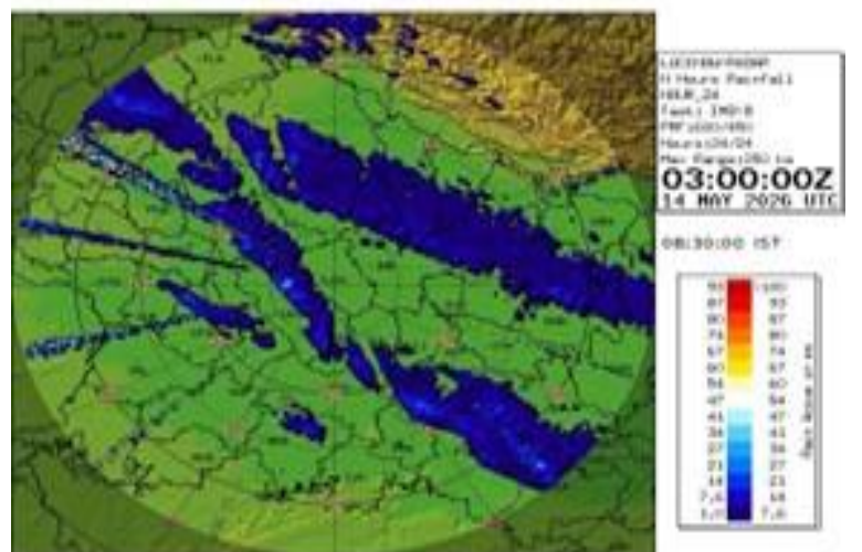
Fig-4(a-h): RADAR Images of Thunderstorm Event
