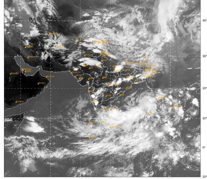
Fig-5(a-f): Typical Satellite Imageries showing thunderstorm clouds over UP on 13 May 2026
