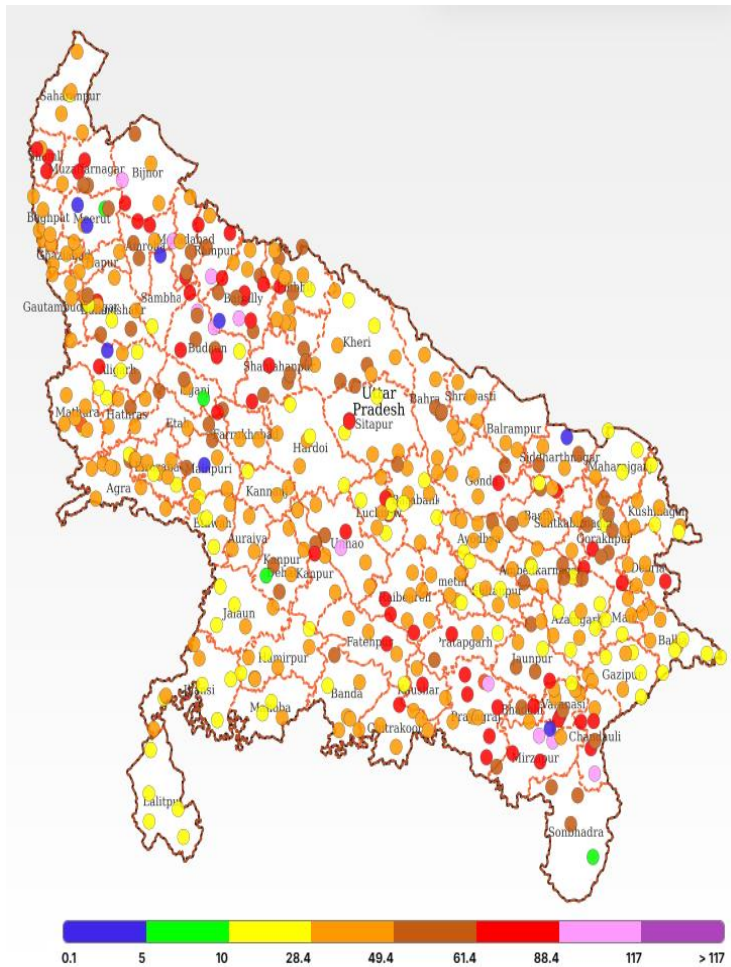
Fig-2: Realized Peak Gusty wind speed over UP
