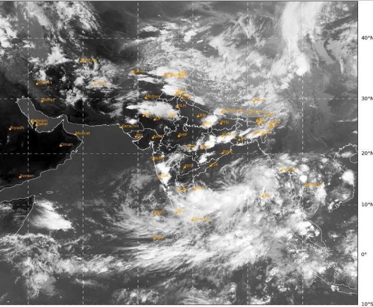
Fig-5(a-f): Typical Satellite Imageries showing thunderstorm clouds over UP on 13 May 2026
